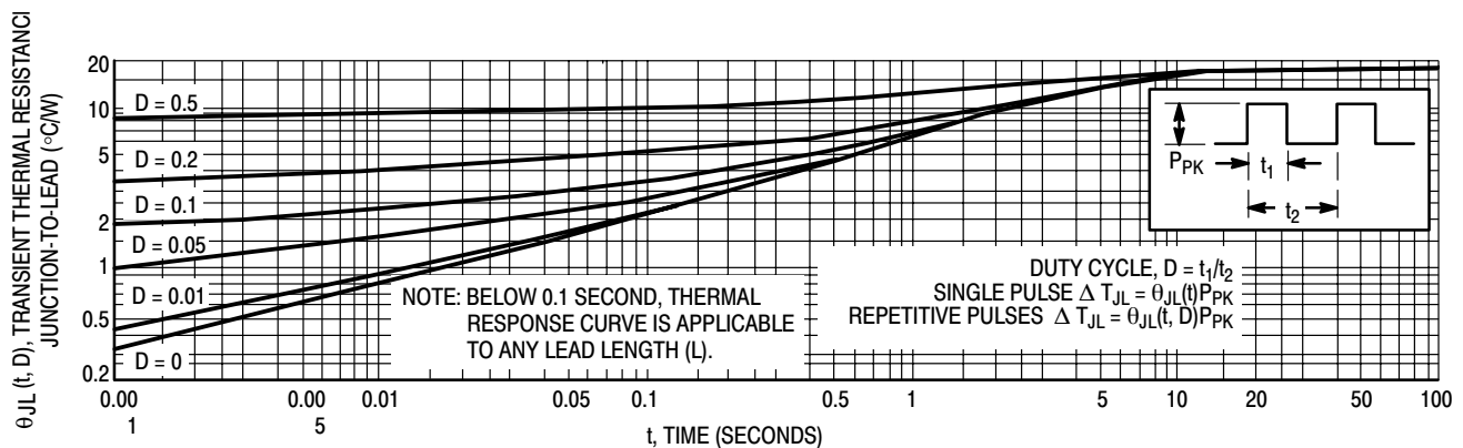
Figure 4. Typical Thermal Response L, Lead Length = 3/8 Inch
