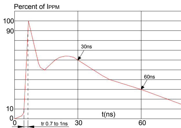
FIG.4: ESD clamping (22kV contact)
