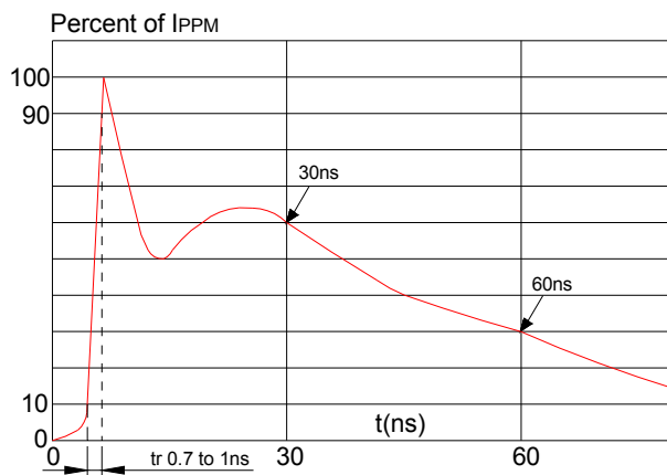
FIG.4: ESD clamping (8kV contact)
